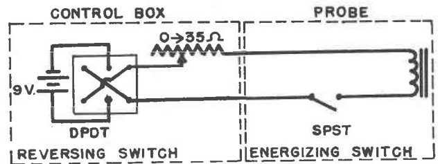
FIG. 1. Schematic wiring diagram for hand-held electromagnet-probe.
